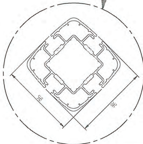
Multipole 250x250 TRIO
